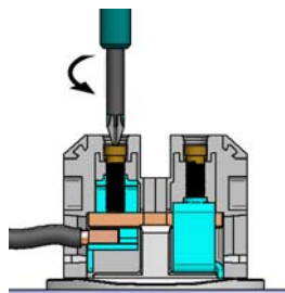
Figure 6: Fixing the supply cable.
